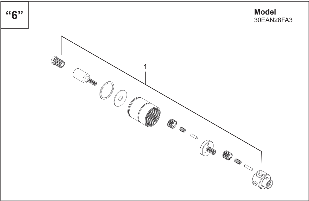
Illustration "6": 302109PT Double Stage Gearing
