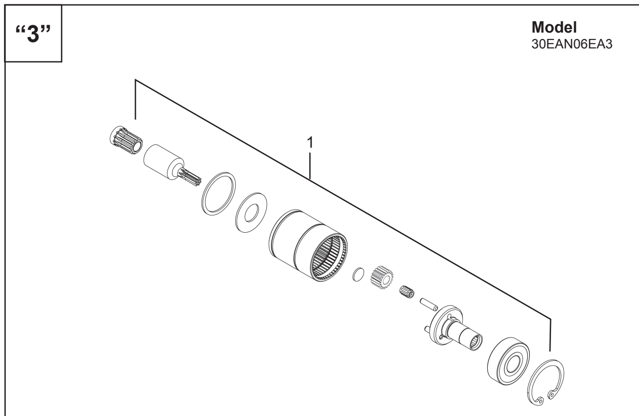
Illustration “3”: 302192PT Single Stage Gearing
