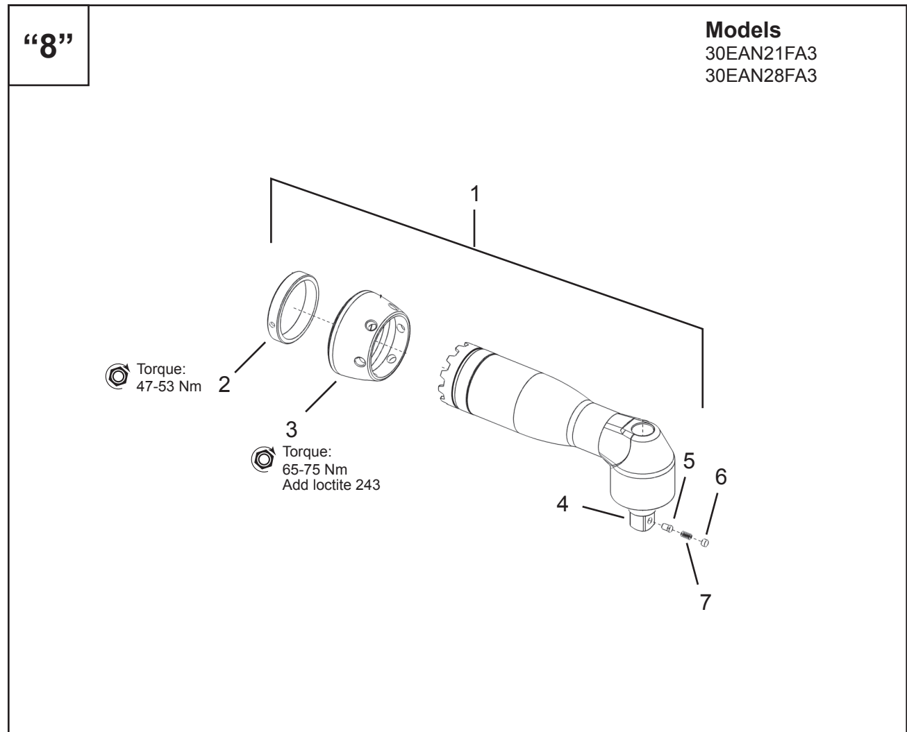
Illustration “8”: 302172PT Angle Head Attachment (FA3)
