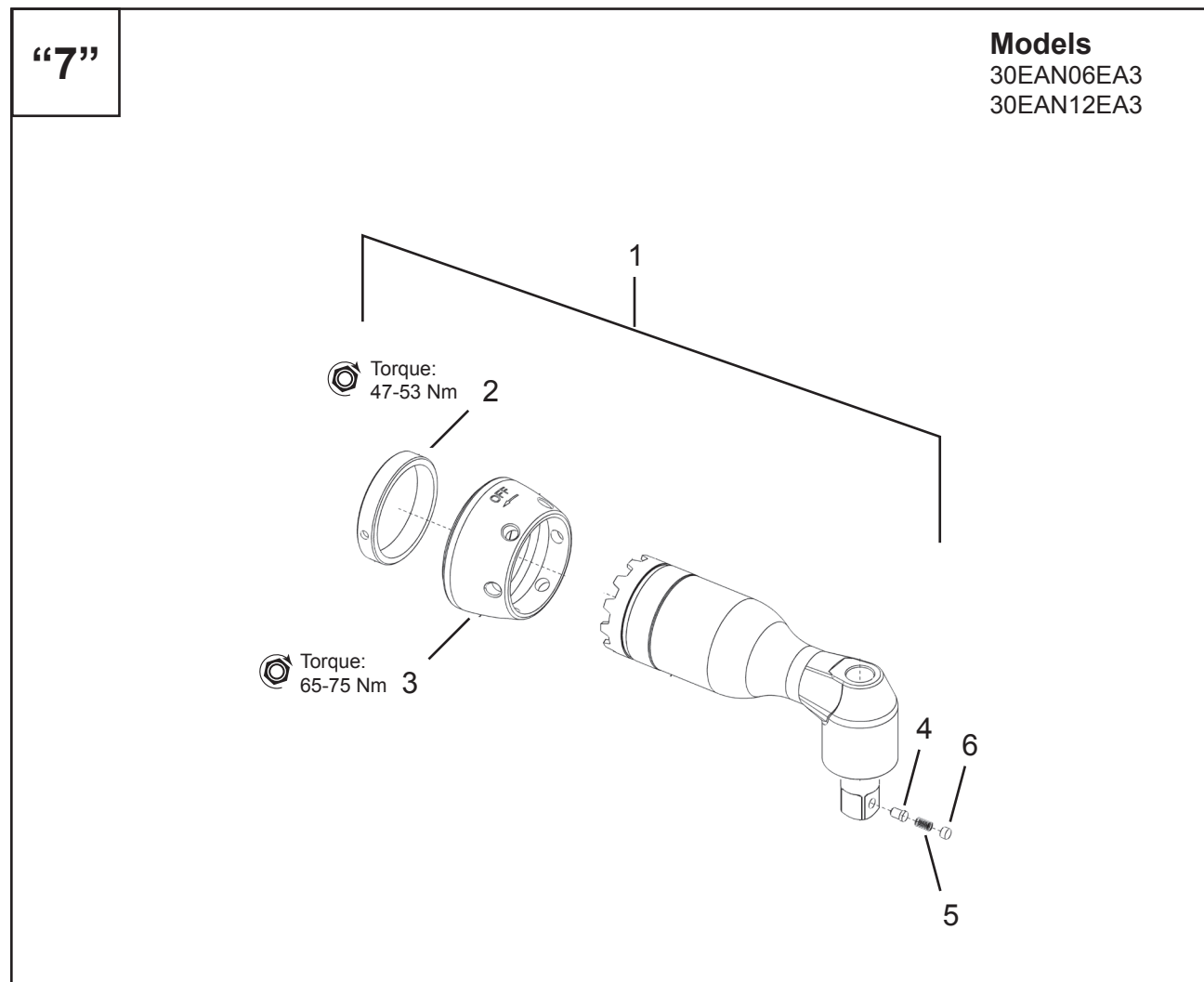
Illustration “7”: 302102PT Angle Head Attachment (EA3)
