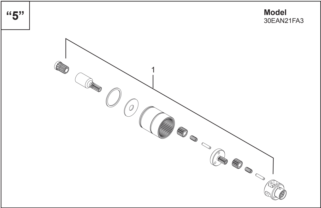
Illustration "5": 302145PT Double Stage Gearing
