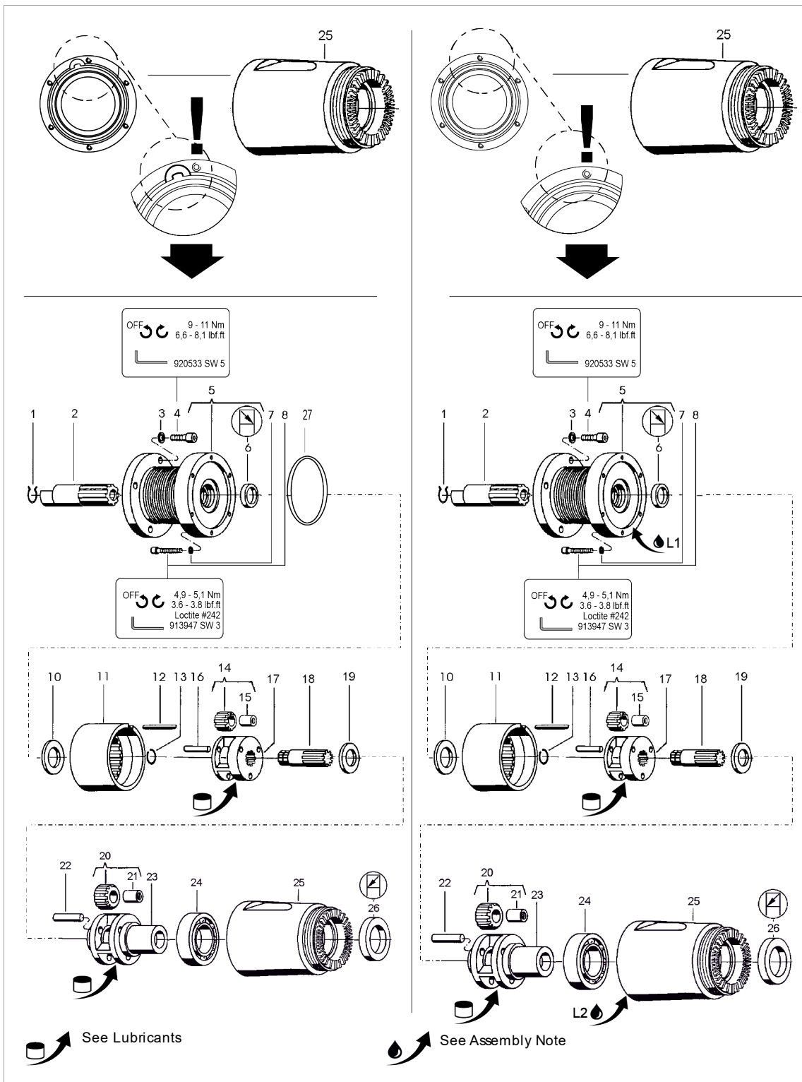
Fig. 4-1: Assembly 3B300A
