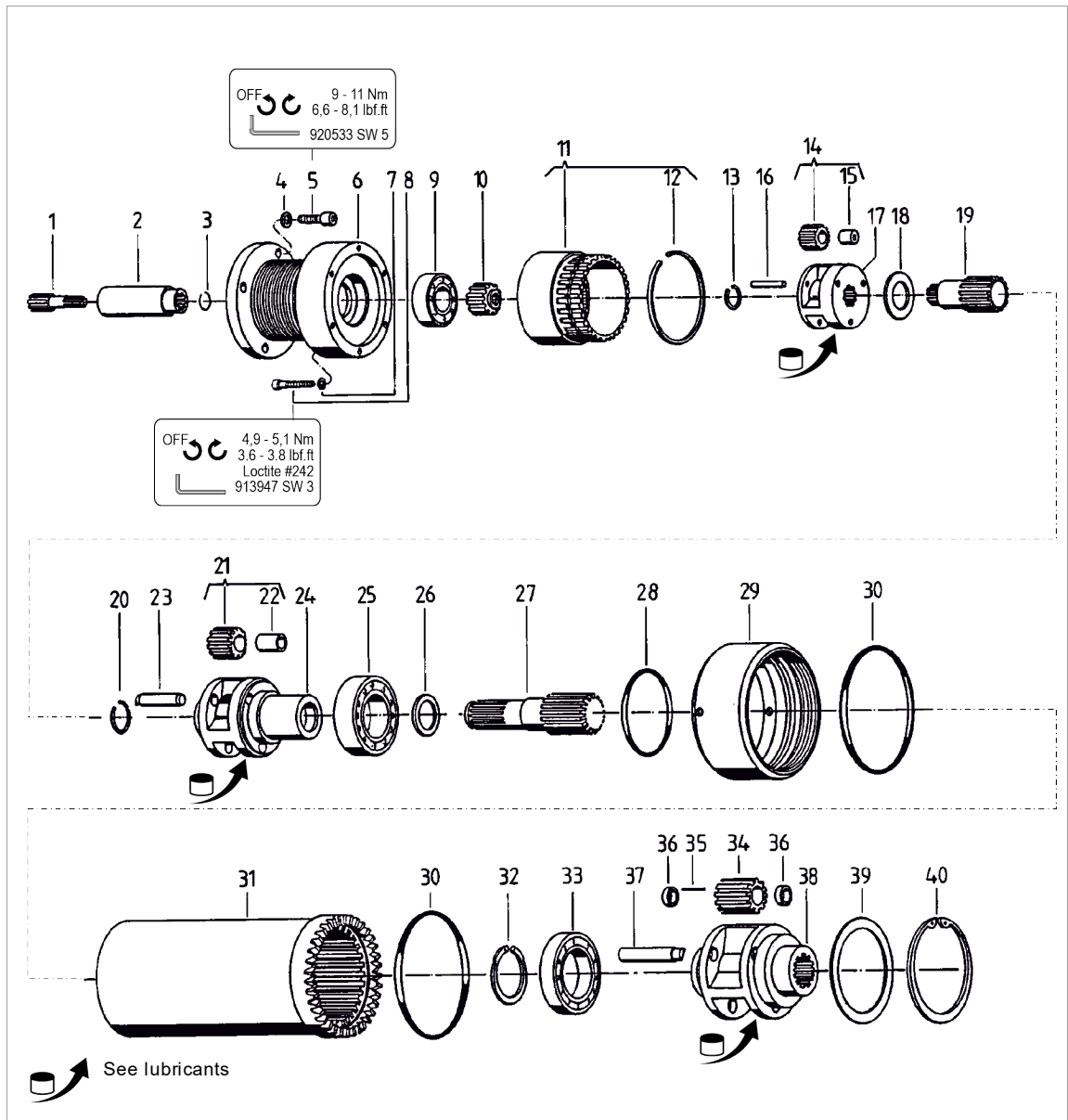
Fig. 5-2: Assembly 4B660A
