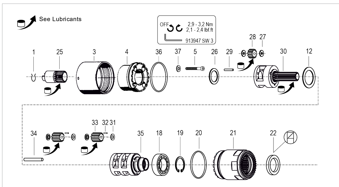
Fig. 3-2: Assembly 2B200A
