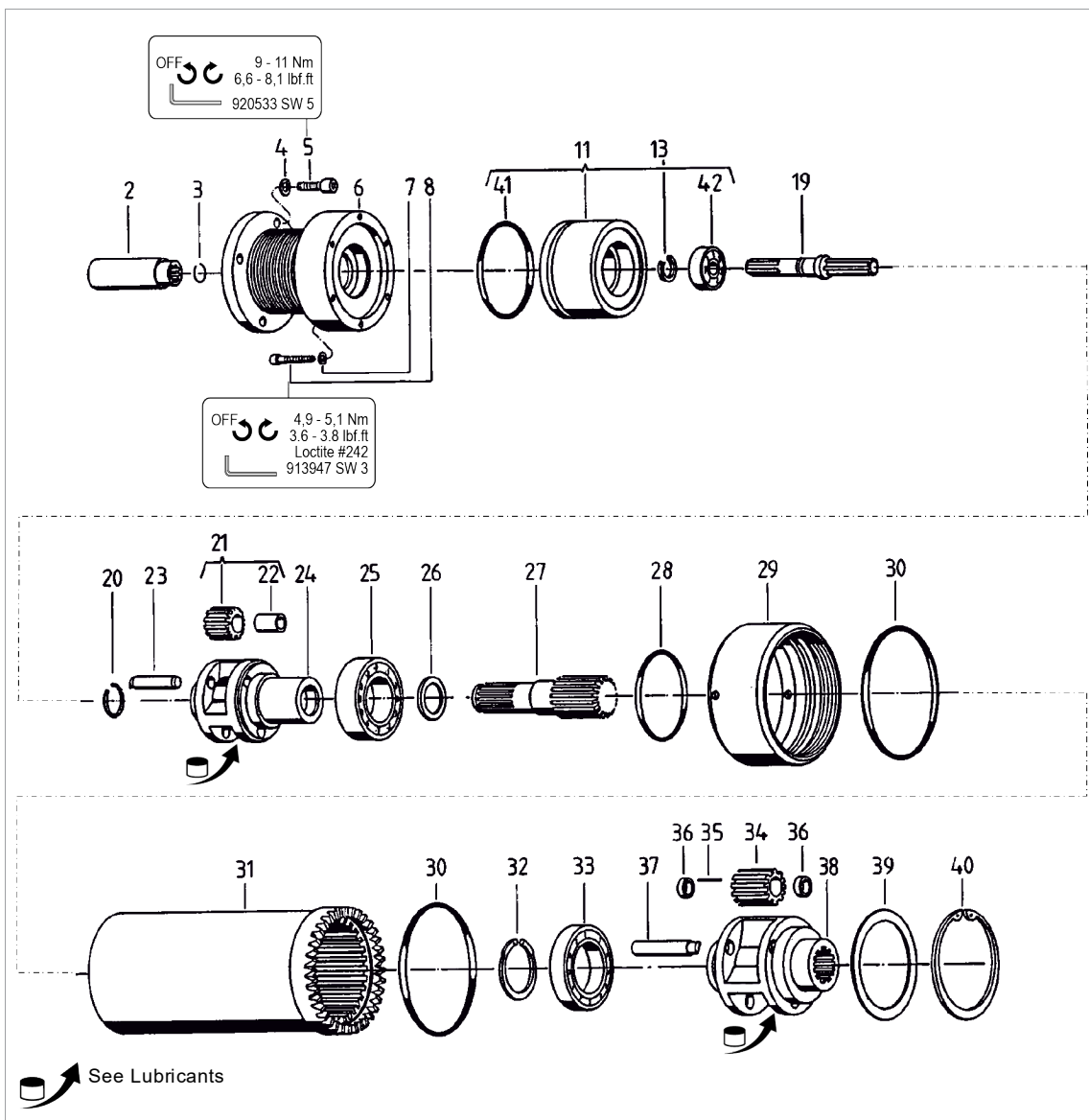
Fig. 5-1: Assembly 4B360A / 4B500A
