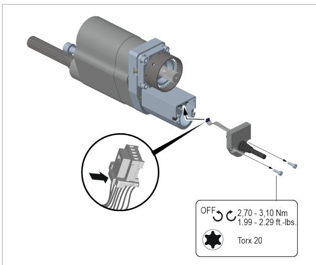
Fig. 1-1: Replacing the cable
