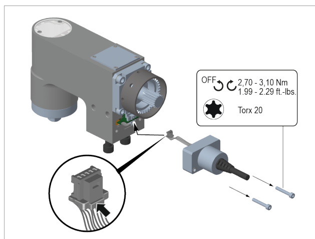
Fig. 1-1: Replacing the cable
