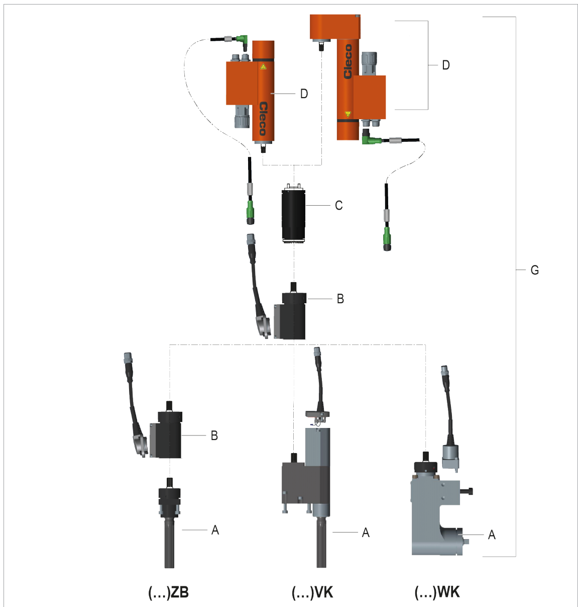
Fig. 3-2: Components, size 1 shown
